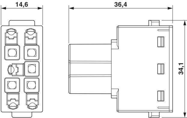
Dimensional drawing
